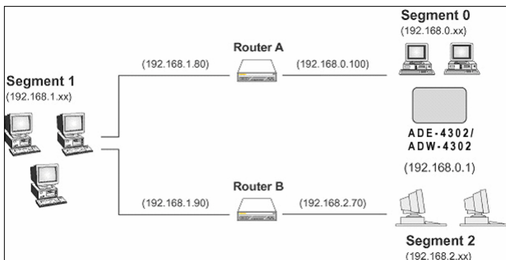
Figure 91: Routing Example
